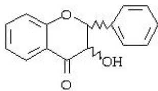
3-Hydroxy flavanon
