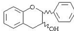
Flavan-3-ol
