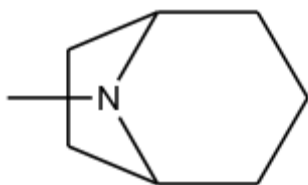
tropan
