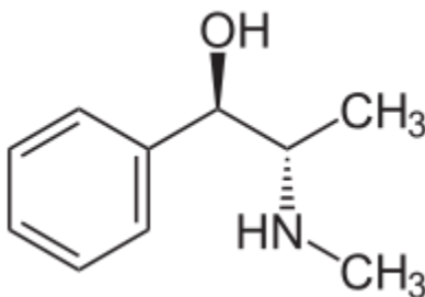
Ephedrin
