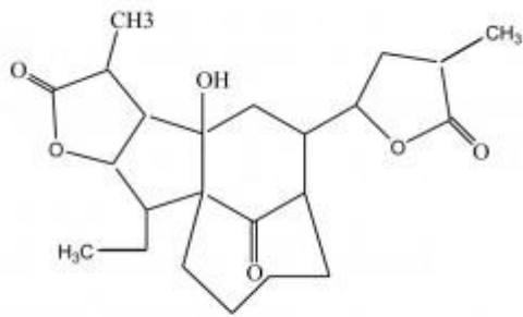
tuberostemoninol
