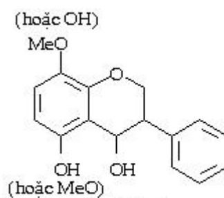
Lapathinol
