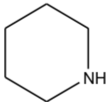
piperidin
